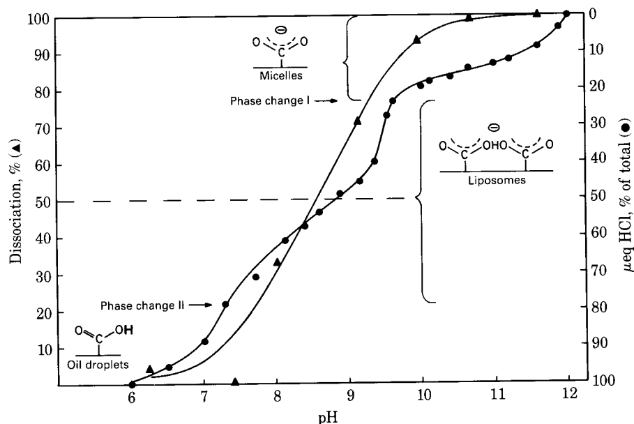
FIG. 1. Titration of a dispersion of 50 mM oleic acid and 10 mM [ 1\text{-}^{13}\text{C} ]lauric acid from pH 12 to pH 6. ^{13}\text{C} NMR experiments were performed on a Varian CFT 20 20-MHz spectrometer in pulse-Fourier transform mode. Most spectra were obtained after 30,000 transients. The chemical shift of the labeled carbon is sensitive to the protonation state of the carboxylate. The percent of total chemical shift in ppm is directly proportional to the percent dissociation of carboxylate. The percent total shift is plotted against pH (▲). For comparison, a titration plotting the percent of total HCl required for complete protonation vs. the pH is shown (●). This titration displays two inflection points, at pH 9.45 and 7.15. The higher inflection point is associated with a transition from micelles to liposomes; the lower inflection point accompanies a phase change from liposomes to oil droplets. This titration is essentially that of Hargreaves and Deamer (33); they confirmed the presence of liposomes by interference microscopy. They and Gebicki and Hicks (32) measured the trapped volume of these liposomes. The pK of the fatty acid titration as estimated by NMR is 8.6. Stable liposomes are found between pH 9.5 and 7.2 and are oligolamellar.
