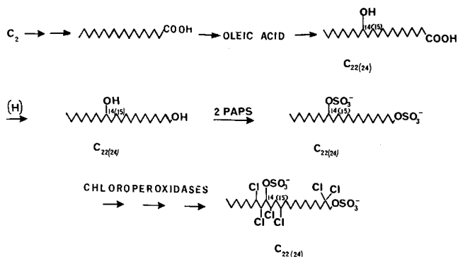
FIGURE 3: Biosynthetic pathway for the chlorosulfolipids of O. danica proposed by Mooney et al. (1972).
