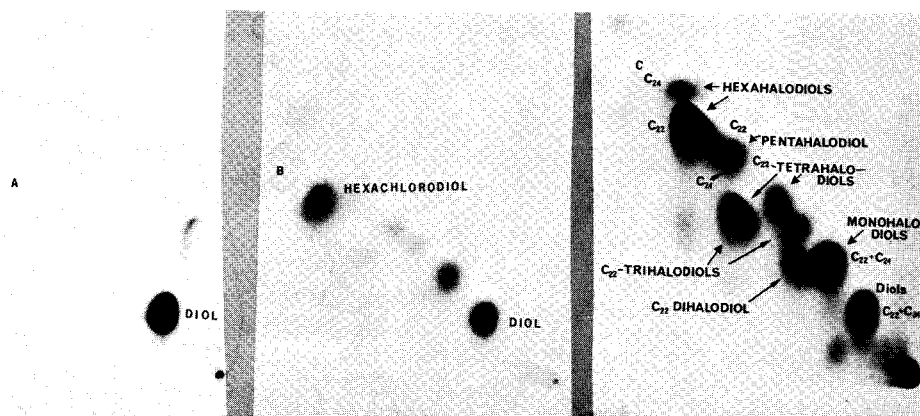
FIGURE 2: Autoradiograms of two-dimensional thin-layer chromatograms of diols obtained by the hydrolysis of sulfatides isolated from O. danica . (a) [1-^{14}\text{C}] Myristate was incubated with the phytoflagellate cultured in halogen-free medium. (b) The sulfatide obtained from the above [1-^{14}\text{C}] myristate feeding was incubated with O. danica cultured in enriched halide medium. (c) [1-^{14}\text{C}] Laurate was fed to the organism grown in normal halide medium. This is the normal diol pattern obtained from O. danica and is shown for comparison purposes. The chromatograms were developed vertically in ether-hexane (3:7, v/v), then horizontally in benzene-chloroform-methanol (50:40:1, v/v/v), and then again vertically in the ether-hexane solvent.
